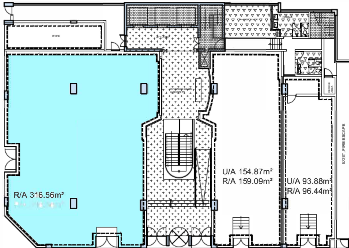
NEDBANK HOUSE - GROUND FLOOR
